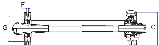
PH2220 series
